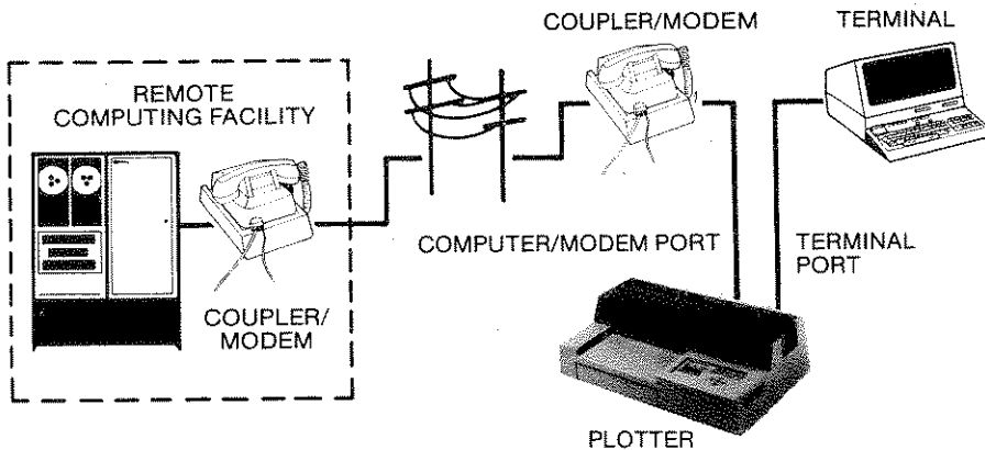
Plotter, Computer, and a Terminal in an Eavesdrop Configuration with Modems
