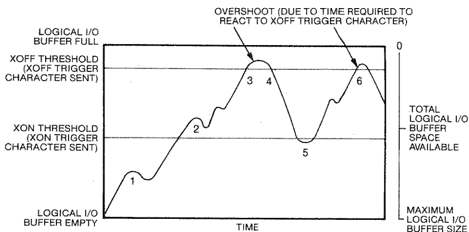
Xon-Xoff Threshold Levels
