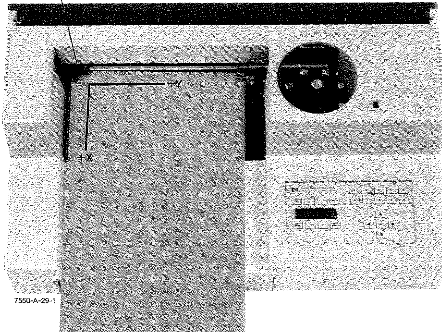
Default Orientation of Plotter Coordinate System (A3/B Paper)
