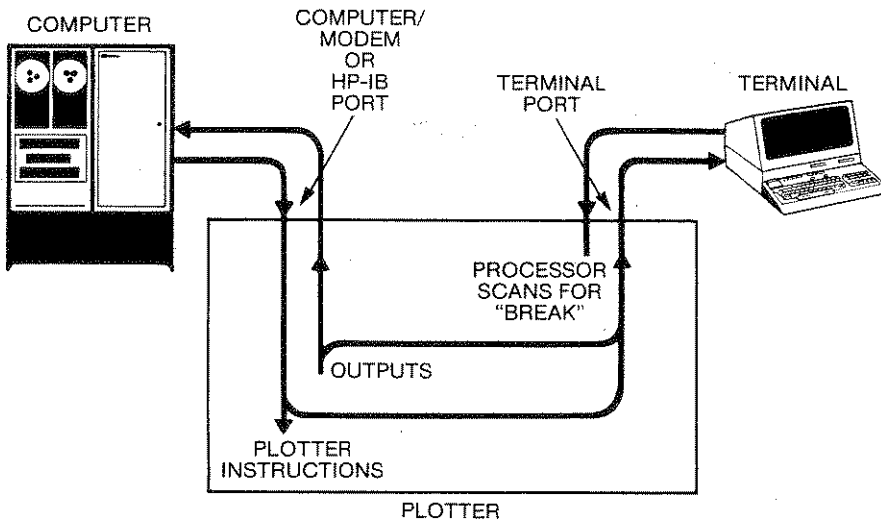
Parse Mode (HP-IB or RS-232-C) and Receive Mode (Half-Duplex RS-232-C)
