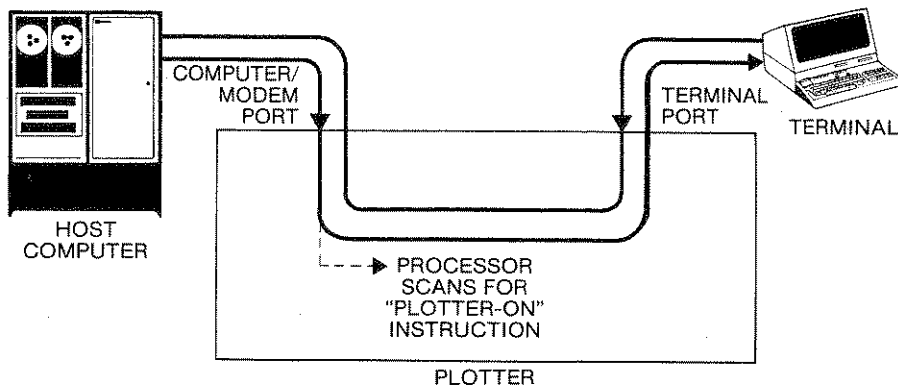
Plotter in Remote Eavesdrop Mode, Programmed-Off
